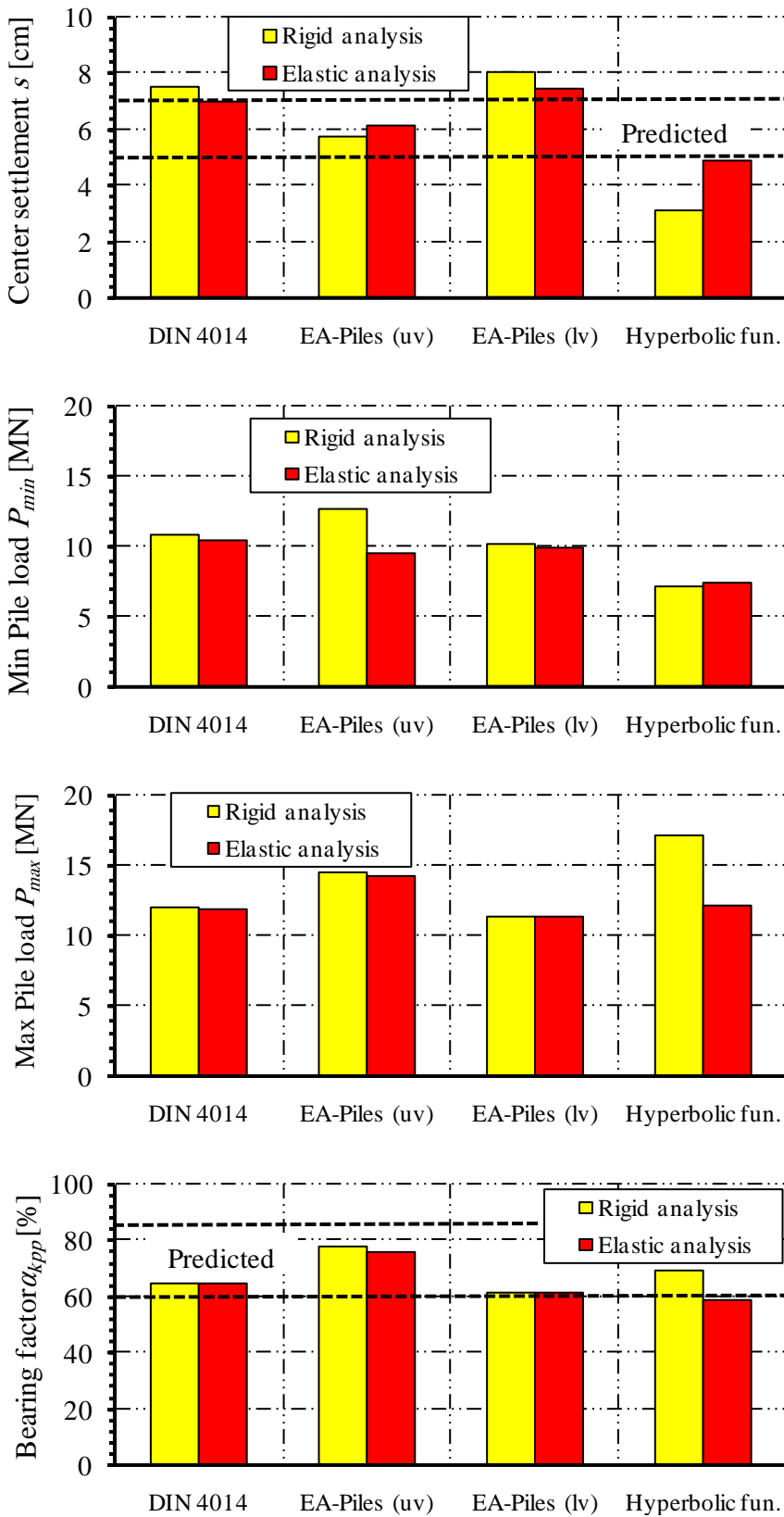
Figure 6-9 Results obtained from measurements and ELPLA
